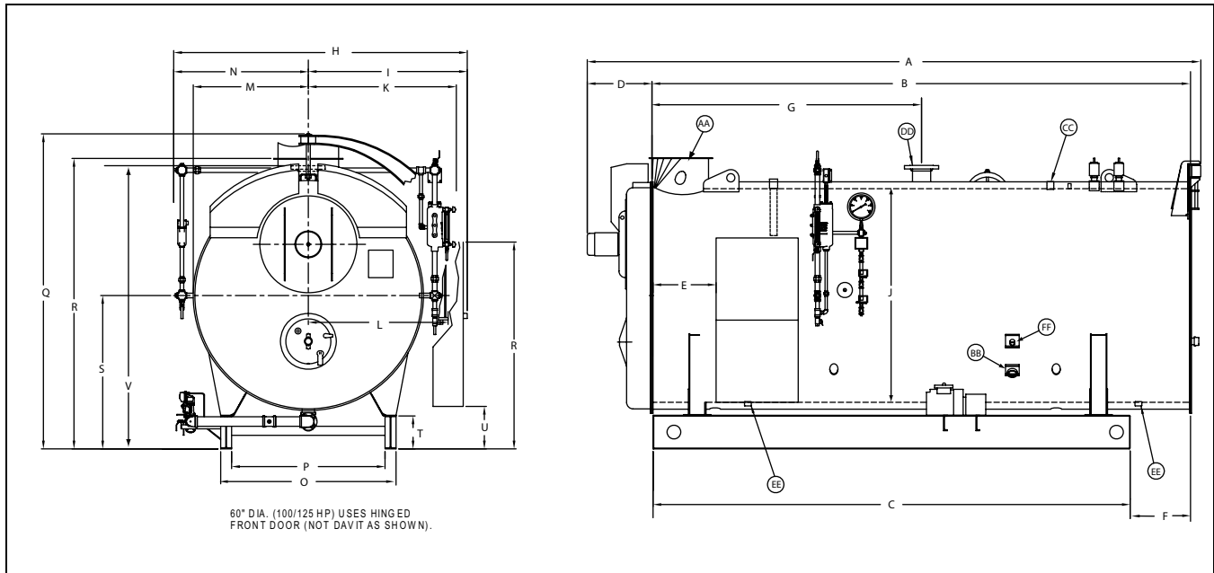
Figure A2-1. Model 4WI Steam Boiler 100-800 HP
