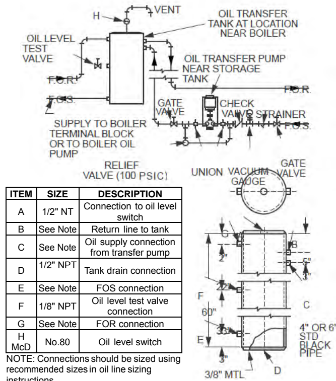
Figure A2-8. No. 2 Oil Transfer Tank Detail (For consideration with elevated boiler rooms)
